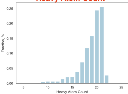
Heavy Atom Count
